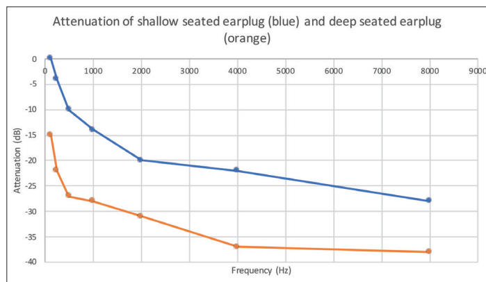
Figure 1. Frequency dependence of a typical foam earplug.
